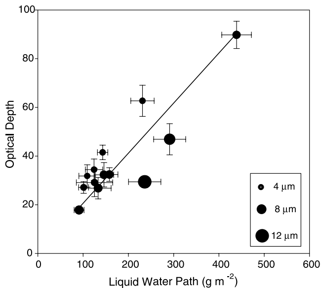
Figure 7. Scatterplot of event-average cloud optical depth ( \tau_c ) against event-average cloud LWP. Radius of filled circles is proportional to effective radius, and error bar indicates 2 times overall uncertainties of cloud optical depth and LWP, respectively. The regression slope of event-average \tau_c vs. event-average LWP constrained through the origin is 0.21 corresponding to r_e of 7.1 \mu\text{m} , and the fraction of the variance ( F ) in \tau_c associated with the regression is 0.74.
