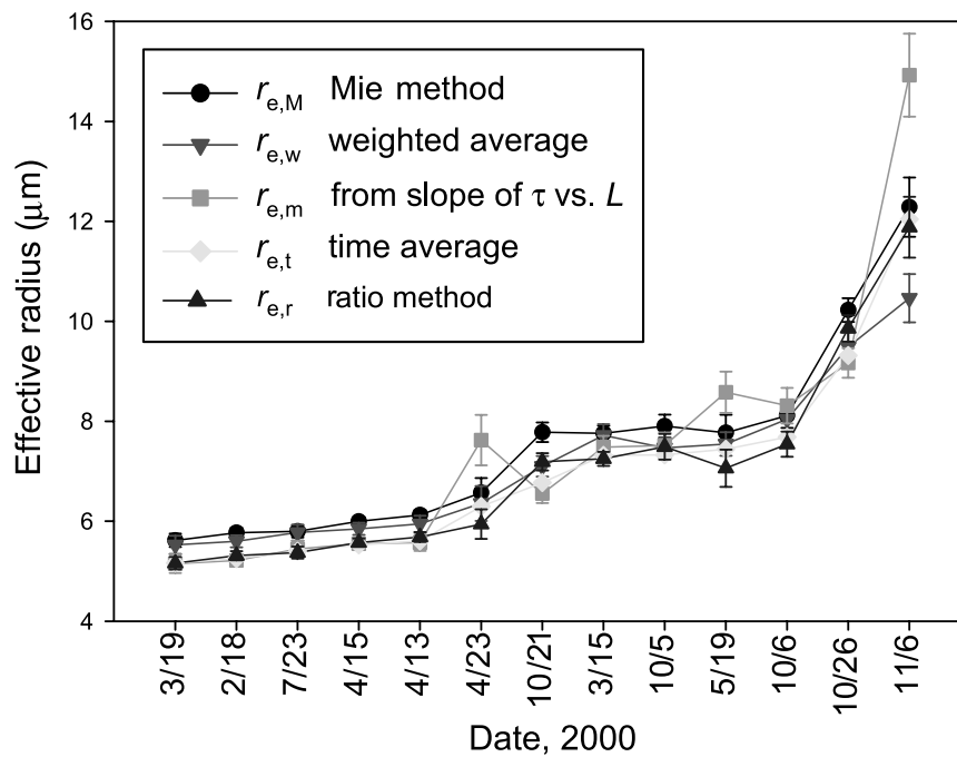
Figure A1. Comparison of alternative approaches to evaluating episode-average cloud drop effective radius: r_{e,M} , from Mie scattering retrieval; r_{e,w} , weighted average of individual measurements of effective radius; r_{e,m} , effective radius obtained from the slope of optical depth vs. LWP; r_{e,t} , ratio of time average LWP to time average optical depth; and r_{e,r} , average of measurements of effective radius evaluated from ratio of LWP to \tau_c , all presented in order of increasing value of r_{e,t} . Error bars indicate the overall uncertainties of indicated quantities. See color version of this figure at back of this issue.
