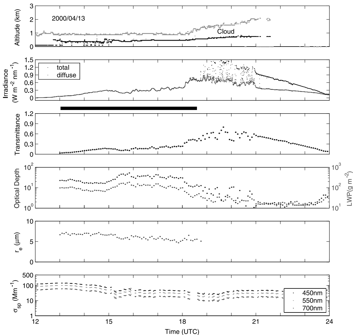
Figure 2. Time series of cloud boundaries (cloud base and cloud top heights), total horizontal and diffuse irradiances, atmospheric transmittance, cloud optical depth ( \tau_c ), LWP, effective radius of cloud droplets ( r_e ) and aerosol scattering coefficient ( \sigma_{\text{sp}} ) on April 13, 2000. Thick black line indicates the period that satisfies the selection criteria for further analysis. See color version of this figure at back of this issue.
