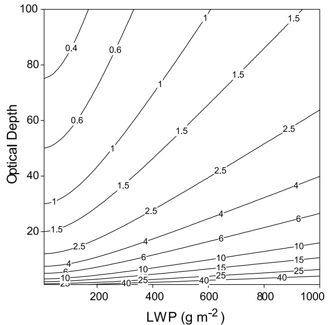
Figure 6. Measurement uncertainties \delta(\overline{r_e}) , \mu\text{m} , associated with a single measurement of r_e as a function of \tau_c and LWP. These uncertainties pertain to retrieval of r_e by equation 6.
