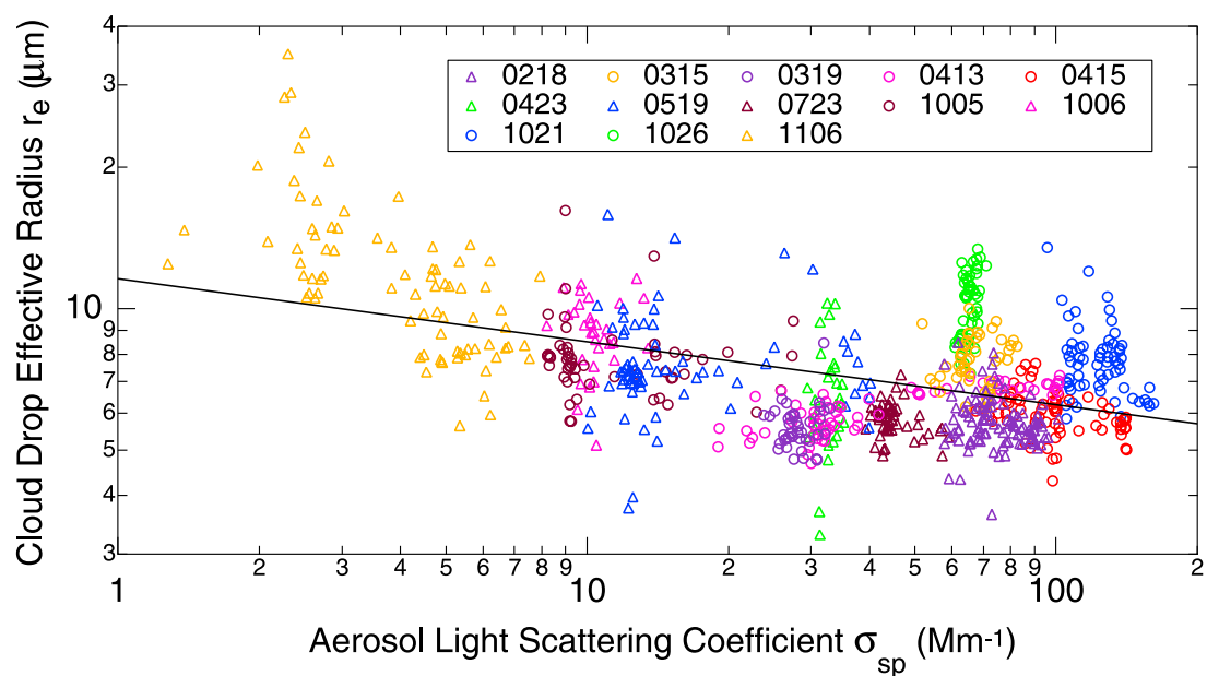
Figure 9. Scatterplot (logarithmic axes) of 5-minute average cloud-drop effective radius ( r_e ) versus light scattering coefficient for submicrometer aerosol at 550 nm ( \sigma_{sp} ). Data for individual days are distinguished by color and symbol. Equation of regression is \log r_e = 1.06 - 0.13 \log \sigma_{sp} ; R^2 = 0.24 . Data for \sigma_{sp} are interpolated to measurement time of r_e , and gaps in \sigma_{sp} (but not r_e ) are filled by interpolation.
