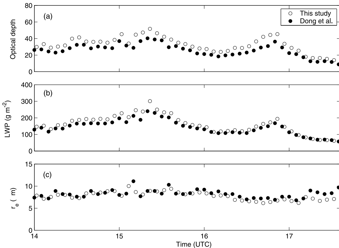
Figure 4. Comparisons of (a) cloud optical depth, (b) LWP, and (c) effective radius on March 15, 2000 with values reported by Dong et al. [2002] for which optical depth was obtained from broadband radiometry and LWP was obtained by the algorithm of Liljegren et al. [2001].
