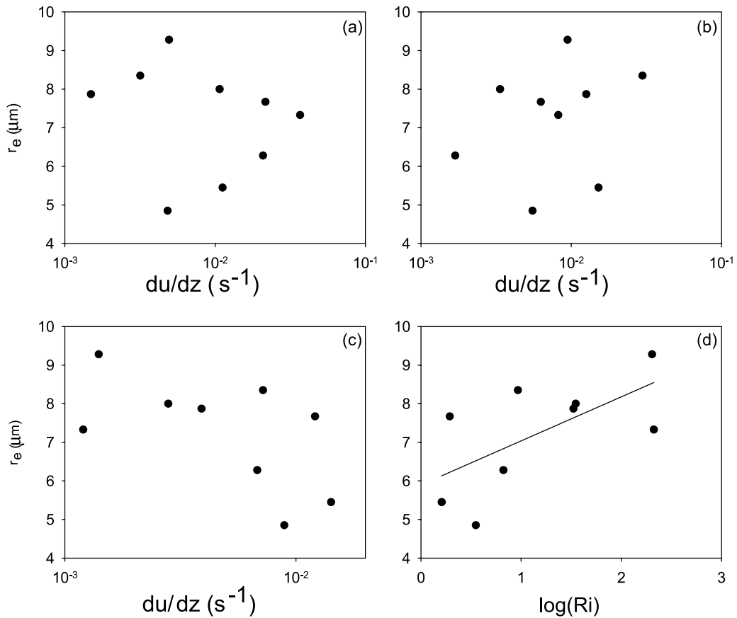
Figure 10. Scatterplots of effective radius versus vertical wind shear for the different layers, (a) below the cloud from the surface to cloud base, (b) in the cloud layer from the cloud base to cloud top and (c) above the mixed layer from the mixed layer to 1 km above the ML top ( R^2 = 0.35 ). (d) Scatterplots of effective radius versus logarithm (base 10) of the Richardson number ( Ri ) above the mixed layer only ( R^2 = 0.41 ).
