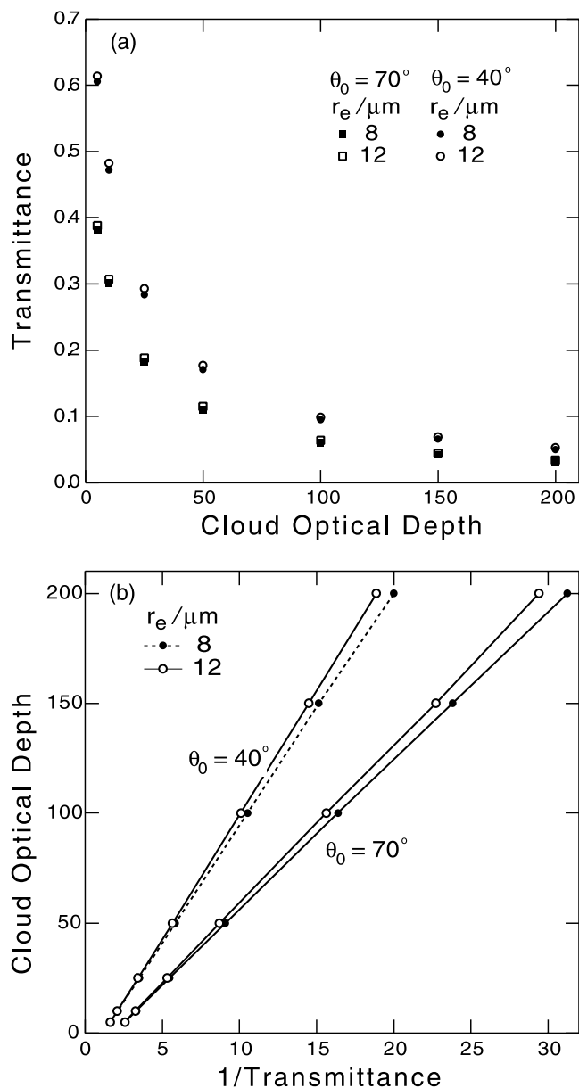
Figure 1. (a) Calculated atmospheric transmittance as a function of cloud optical depth, evaluated as ratio of downwelling irradiance at surface to that at top of atmosphere. (b) Calculated dependence of cloud optical depth as a function of inverse of atmospheric transmittance; lines in (b) connecting points for which calculations were made show near linear dependence of the relation. Wavelength band 0.39\text{--}0.43 \mu\text{m} ; solar zenith angle \theta_0 40^\circ and 70^\circ ; cloud-base height 2 km; surface albedo 0.04; atmospheric water vapor column 2.9 \text{ g cm}^{-2} ; cloud droplet effective radius 8 \mu\text{m} and 12 \mu\text{m} . Calculated with SBDART [Ricchiazzi et al. , 1998; http://arm.mrcsb.com/sbdart/ ].
