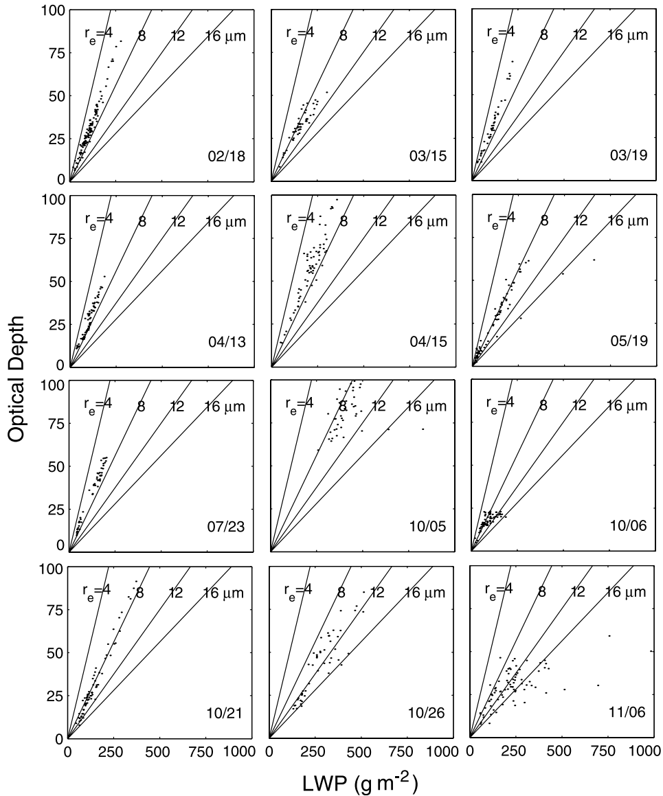
Figure 5. Scatterplots of cloud optical depth ( \tau_c ) against cloud LWP for the analysis period on the different days. Lines denote cloud optical depth for indicated constant values of effective radius, r_e . Scatterplot for April 23, similar to others shown, is omitted from the figure for compactness of presentation.
