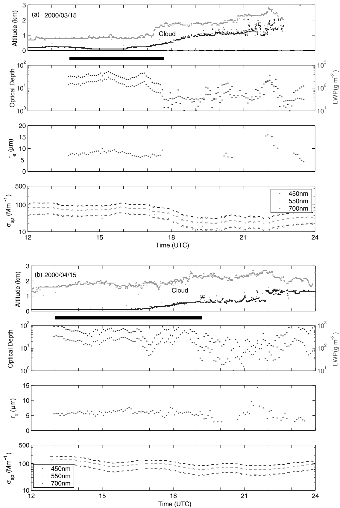
Figure 3. Time series of cloud boundaries, cloud optical depth ( \tau_c ), LWP, effective radius of cloud droplets ( r_e ) and aerosol scattering coefficient ( \sigma_{\text{sp}} ) on the days of (a) March 15, (b) April 15, (c) October 05, and (d) October 26, 2000. Thick black line indicates the period that satisfies the selection criteria for further analysis. See color version of this figure at back of this issue.
