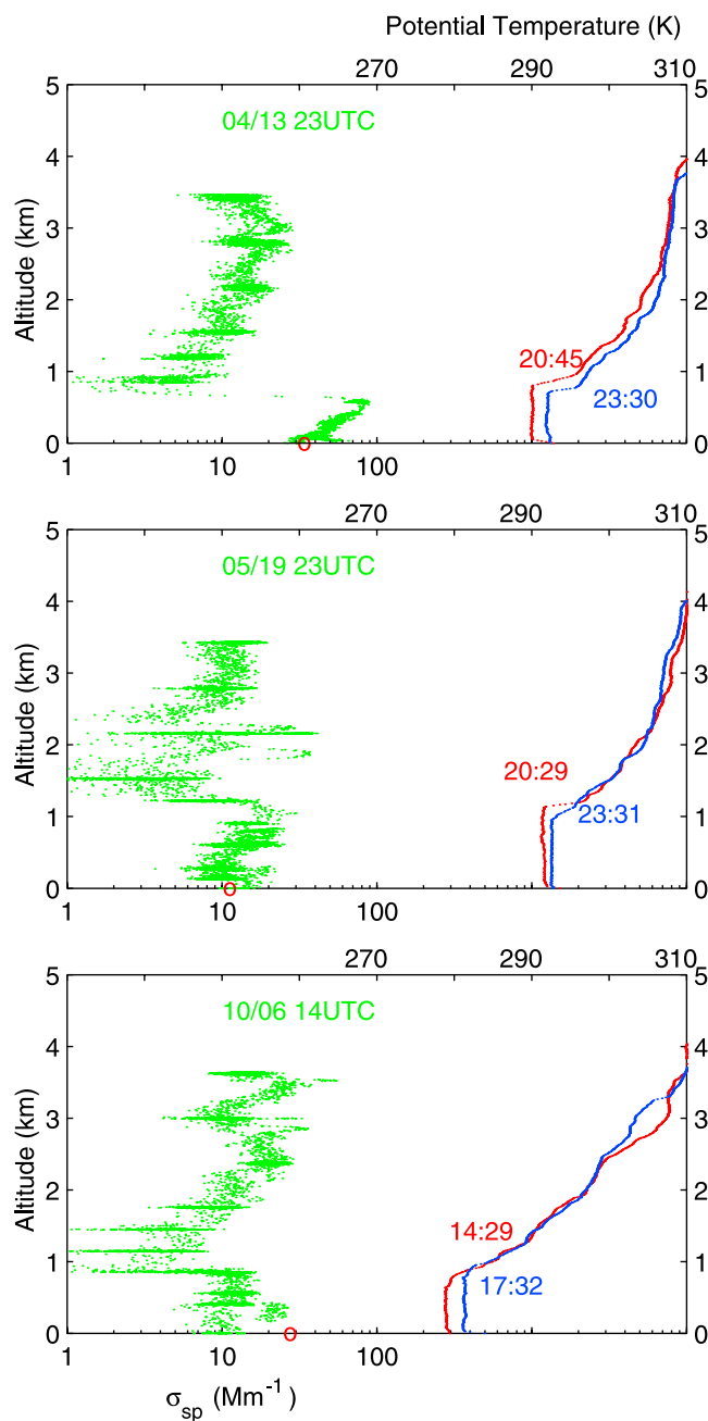
Figure 8. Vertical profiles of aerosol scattering coefficients from in-situ Aerosol Profile (IAP) flights and potential temperature from Balloon-Borne Sounding System (BBSS) on April 13, May 19, and October 6, 2000. Red circle indicates the aerosol scattering coefficient measured at the surface.
