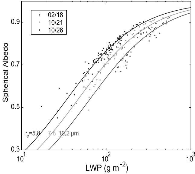
Figure 11. Cloud top spherical albedo as a function of cloud LWP calculated for measured LWP and \tau_c for February 18, October 21, and October 26. Curves denote cloud albedo for indicated constant values of effective radius, r_e . See color version of this figure at back of this issue.
