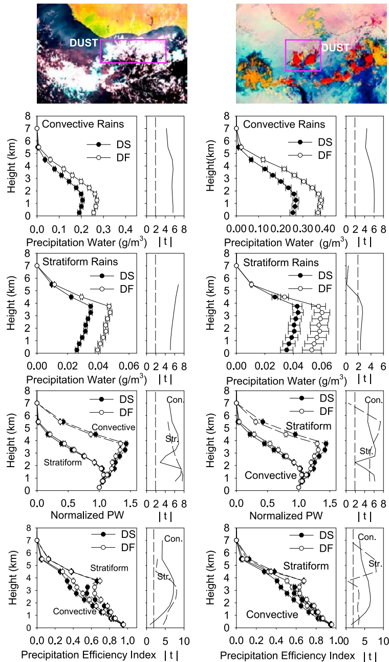
Figure 11. Two other case studies using AMSR-E data. The RGB composite of satellite images taken by Meteosat-8; the mean precipitation water profiles for convective rains; the mean precipitation water profiles for stratiform rains; the normalized precipitation water (PW) profiles for both convective (solid) and stratiform (dashed) rains; and the PEI profiles for both convective (solid) and stratiform (dashed) rain in DS and DF sector in these two cases are given. The t testing significances of difference are also shown (dashed line indicates the 95% confidence level at 60 degrees of freedom).
